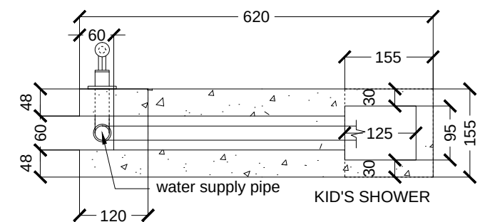
PLAN SCALE 1:10
