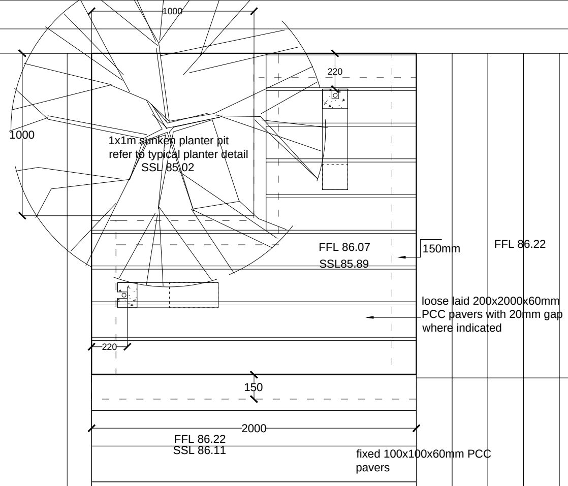
MP DETAIL PLAN : shower area Scale 1:25
