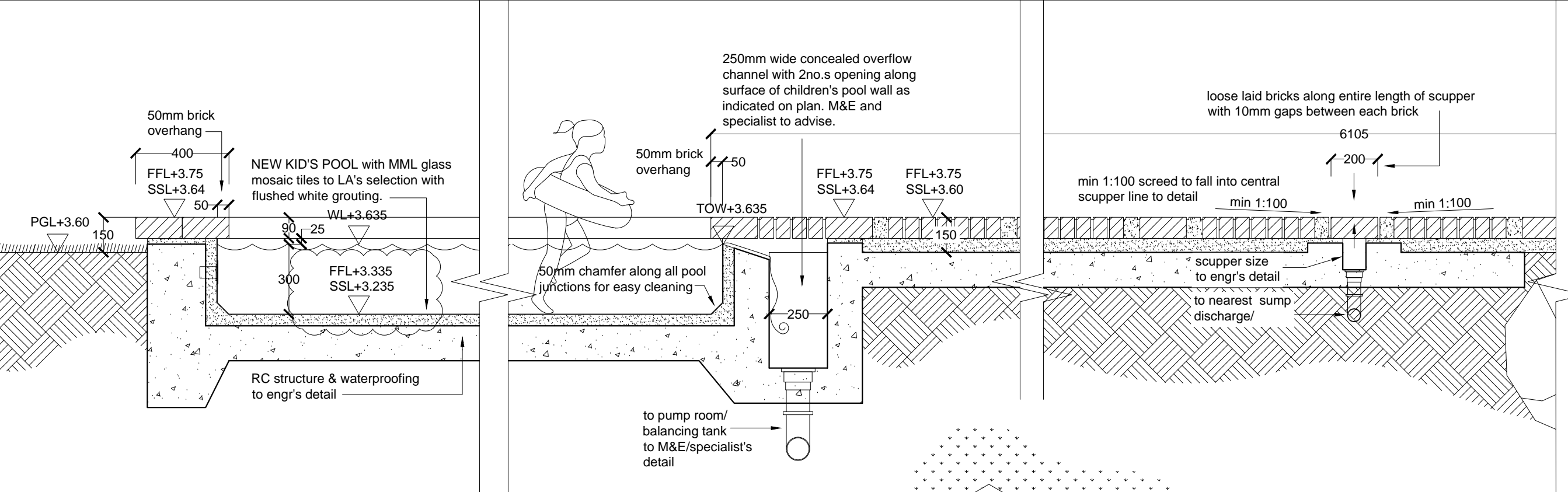
DETAIL SECTION A Scale 1:100
