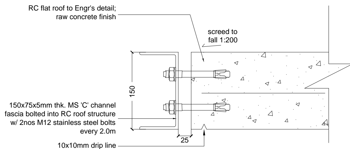
TYPICAL DETAIL B :PAVILLION RC ROOF SCALE 1:5
