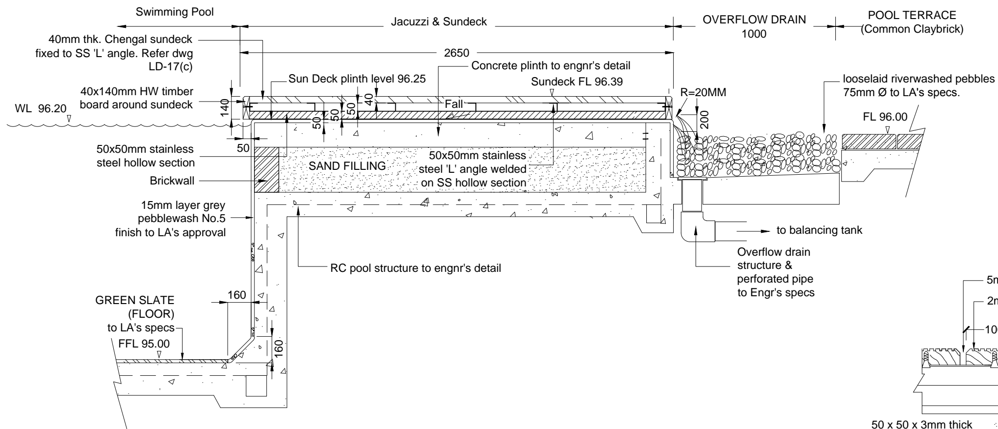
SECTION C Scale 1:25
