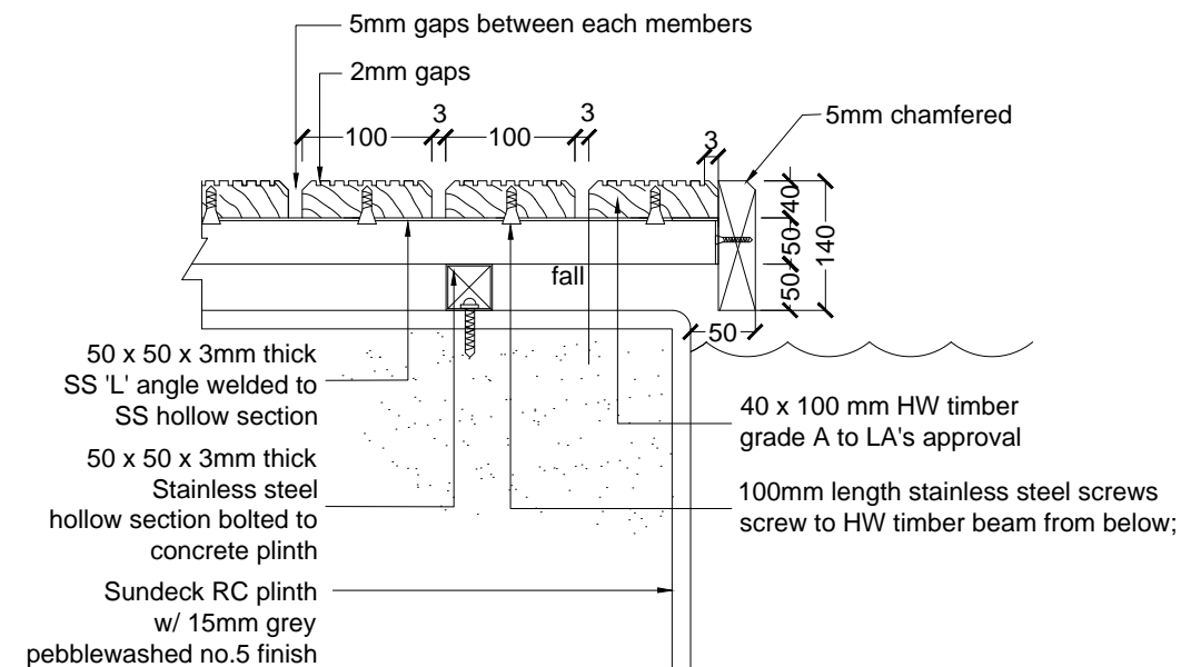
c DETAIL: ANTI-SLIP GROOVED TIMBER DECKING BOARDS
