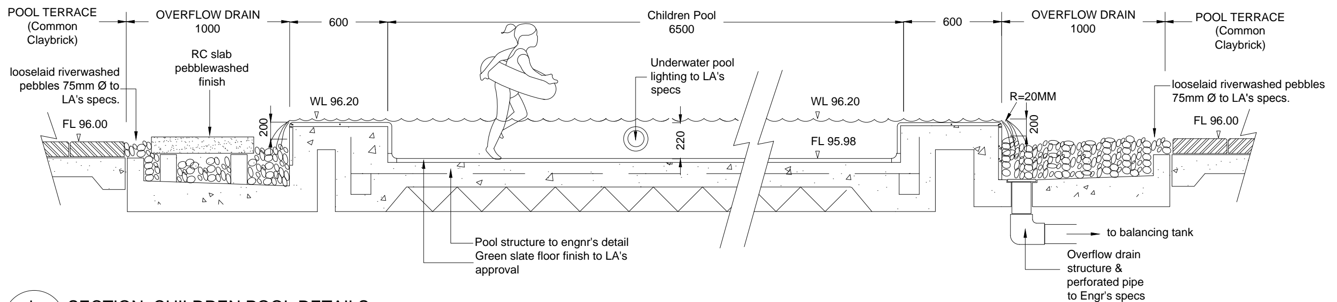
b SECTION: CHILDREN POOL DETAILS
